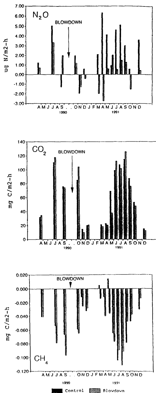
Fig. 1. Fluxes of \text{N}_2\text{O} , \text{CO}_2 , and \text{CH}_4 between soils and the atmosphere during the pre-blowdown and post-blowdown periods in the control and blowdown plots at the Harvard Forest. Negative fluxes indicate uptake.
